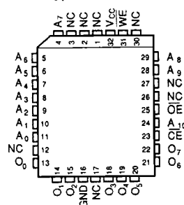
32 Pin PLCC Type "D" Package
