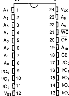
Small Outline Type "J" Package
