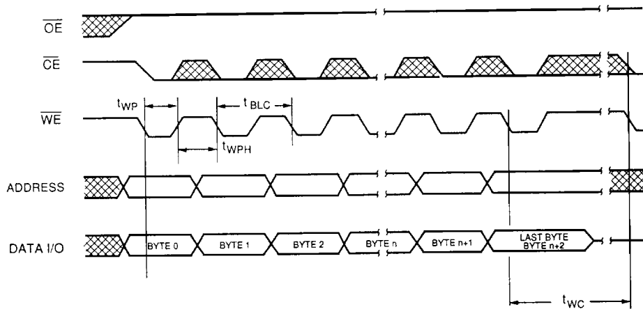
FIGURE 6. PAGE MODE WRITE CYCLE TIMING
