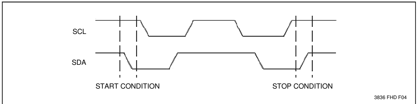
Figure 2. Definition of Start and Stop Conditions
