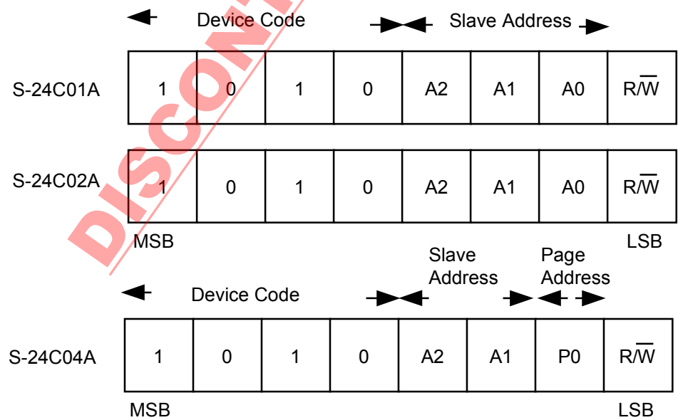
Figure 9 Device Address
