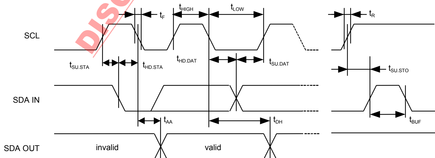
Figure 4 Bus Timing
