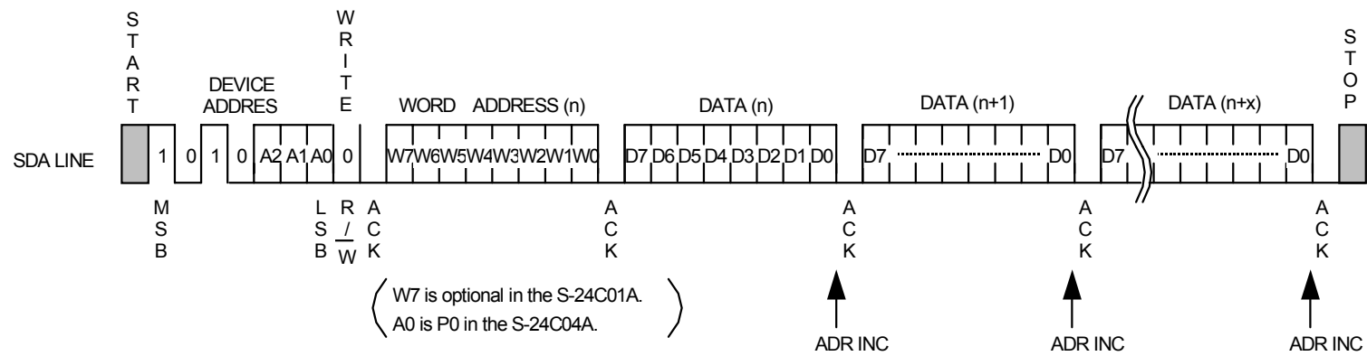
Figure 11 Page Write
