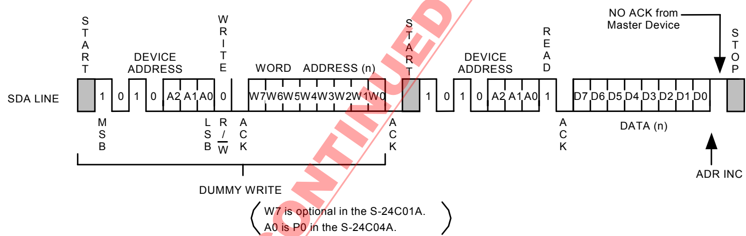
Figure 13 Random Read
