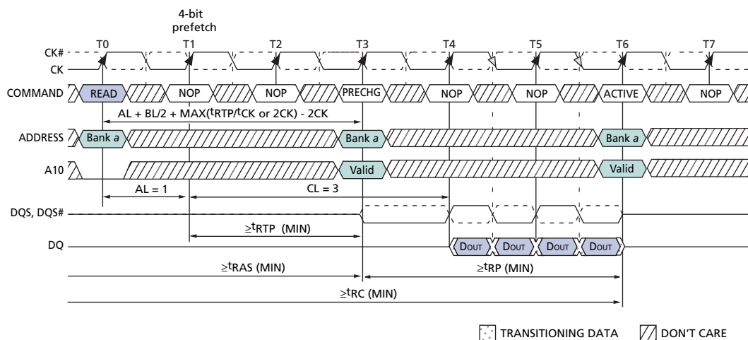
Figure 26: READ-to-PRECHARGE – BL = 4
