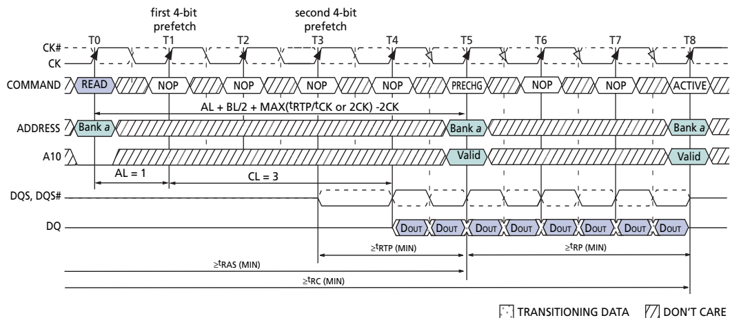
Figure 27: READ-to-PRECHARGE – BL = 8
