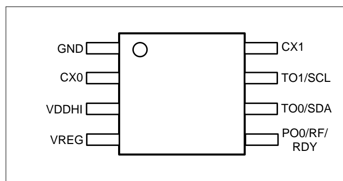
Figure 1.1: IQS232 pin-out.
