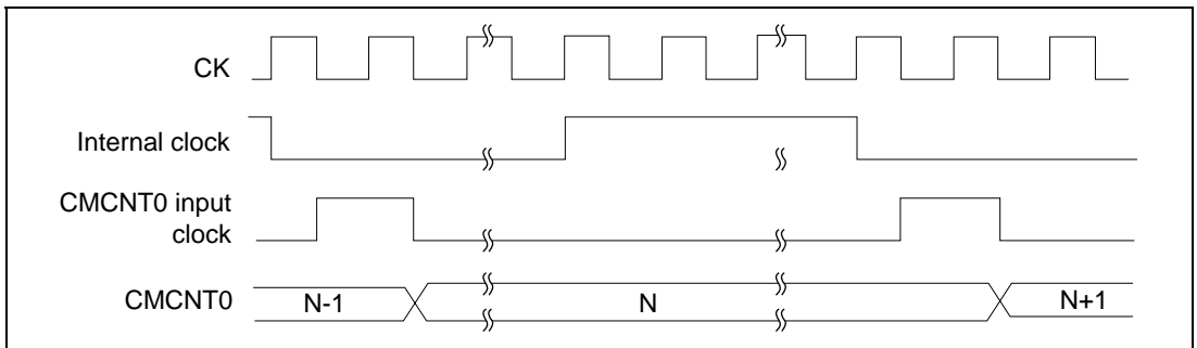
Figure 11.26 Count Timing
