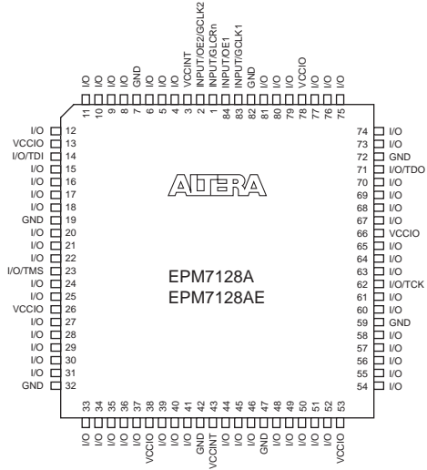
Figure 15. 84-Pin PLCC Package Pin-Out Diagram
