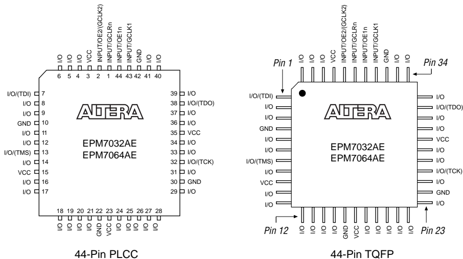
Figure 14. 44-Pin PLCC/TQFP Package Pin-Out Diagram
