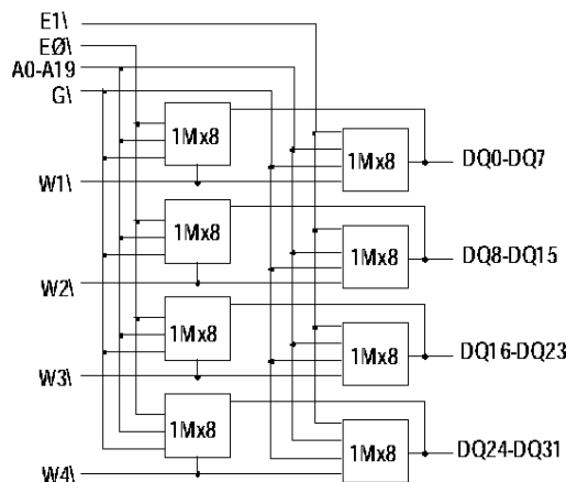
EDI7F2341MV-BNC 2x1Megx32 80 pin SIMM
