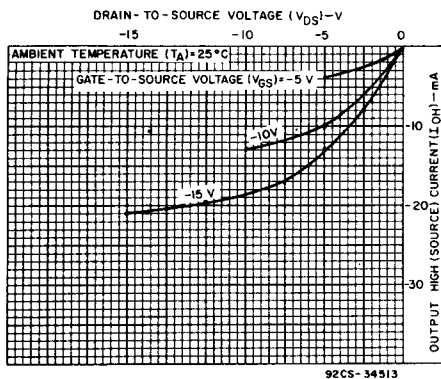
Fig. 2 - Typical output high (source) current characteristics.
