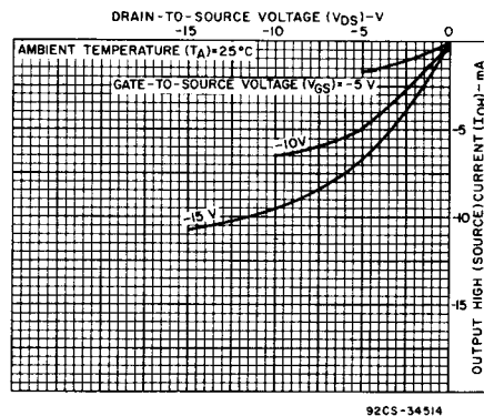
Fig. 3 - Minimum output high (source) current characteristics.
