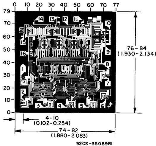
Dimensions and pad layout for CD4543BH.
