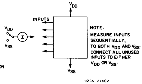
Fig. 12 - Input current test circuit.
