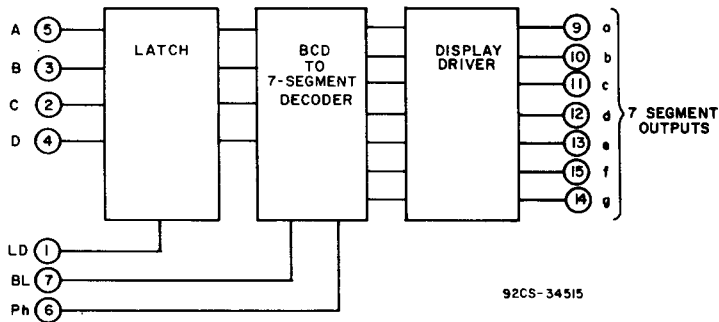
Fig. 4 - BCD-to-seven-segment latch/decoder/driver functional diagram.
