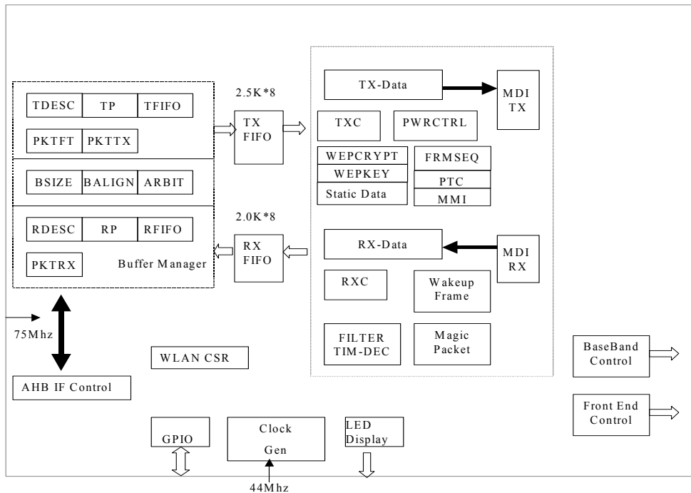
Figure 3-1 Device Functional Blocks
