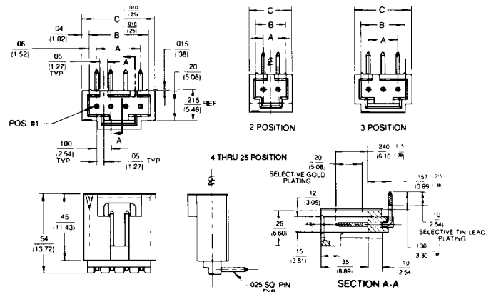
910X-9-1XX-01 Right Angle With Latch
