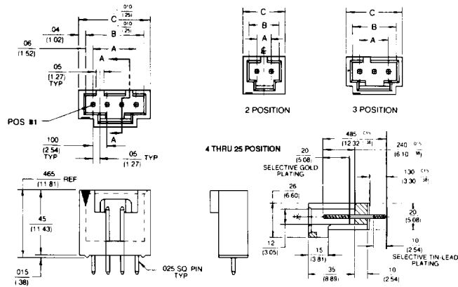
910X-8-1XX-01 Vertical With Latch
