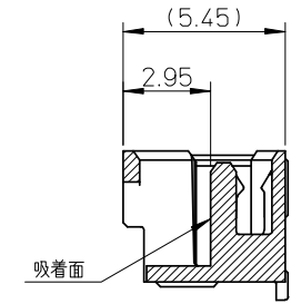
SECTION Y-Y
