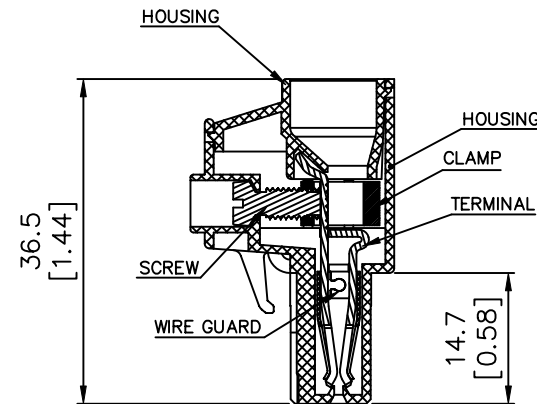
SEC. H-H
