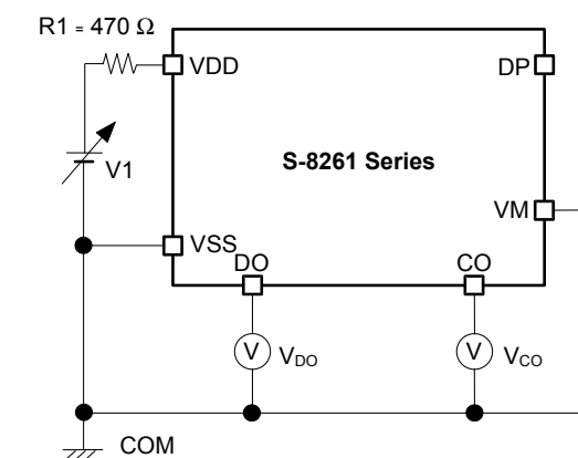
Test Circuit 1
