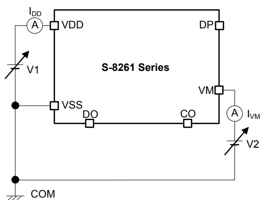
Test Circuit 3
