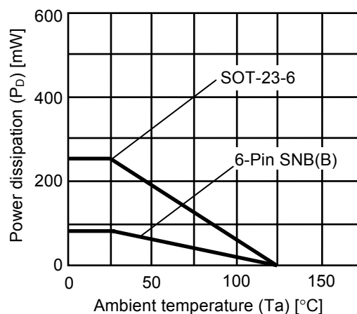
Figure 4 Power Dissipation of Packages (When Not Mounted on Printed Circuit Board)
