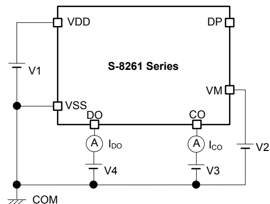
Test Circuit 4
