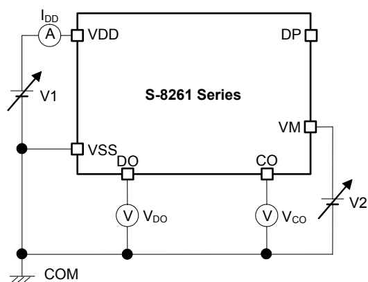
Test Circuit 2
