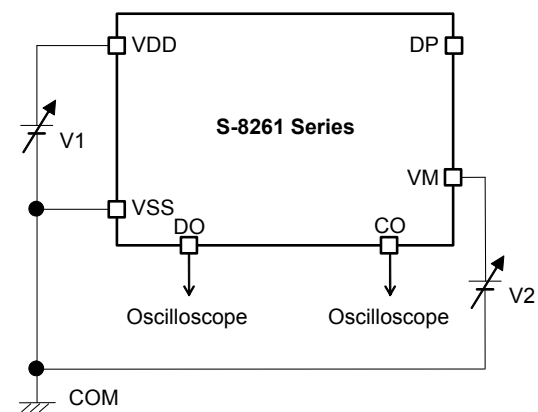
Test Circuit 5
