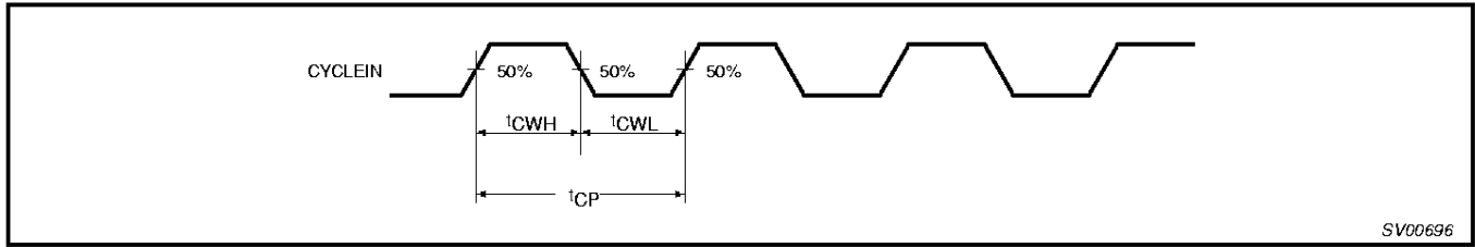
Figure 29. CYCLEIN Waveform
