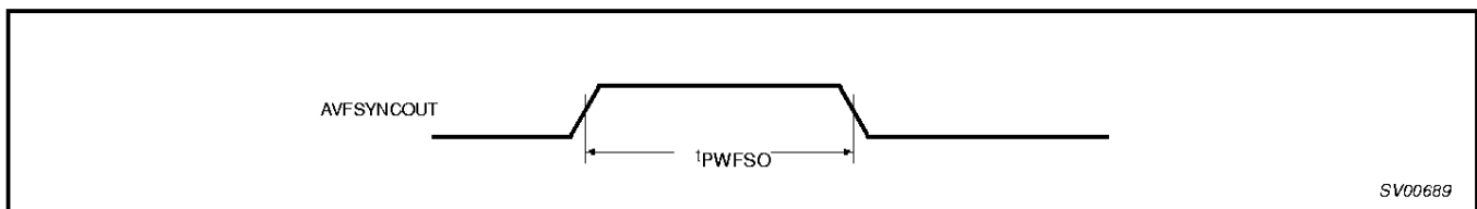
Figure 24. AVFSYNCOU Timing Diagram
