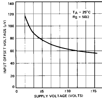
INPUT OFFSET VOLTAGE vs POWER SUPPLY VOLTAGE
