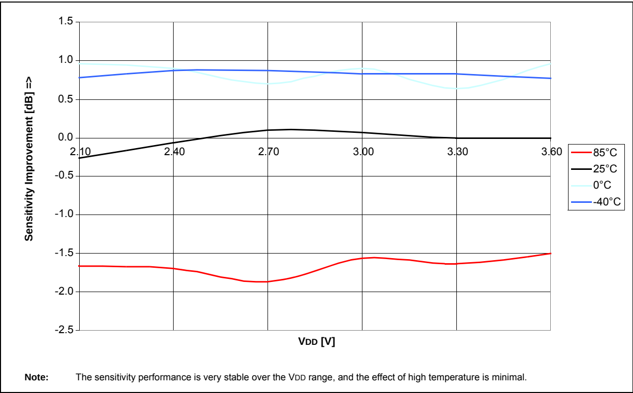
FIGURE 5-12: SENSITIVITY STABILITY
