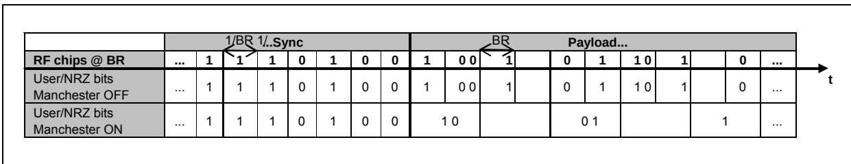
FIGURE 3-30: MANCHESTER ENCODING/DECODING
