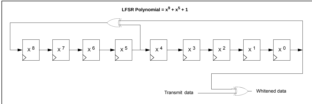
FIGURE 3-31: DATA WHITENING
