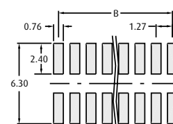
Recommended PC Board Pattern
