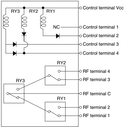
Equivalent circuit
