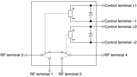
Equivalent circuit
