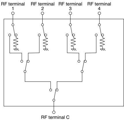
Equivalent circuit
