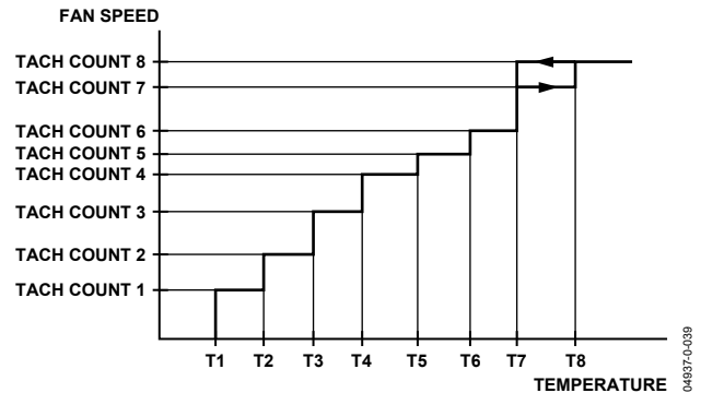
Figure 40. Programming the Look-Up Table in Discrete RPM Mode
