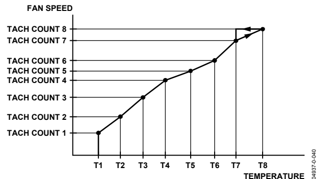
Figure 41. Programming the Look-Up Table in Linear Fan Speeds Mode
