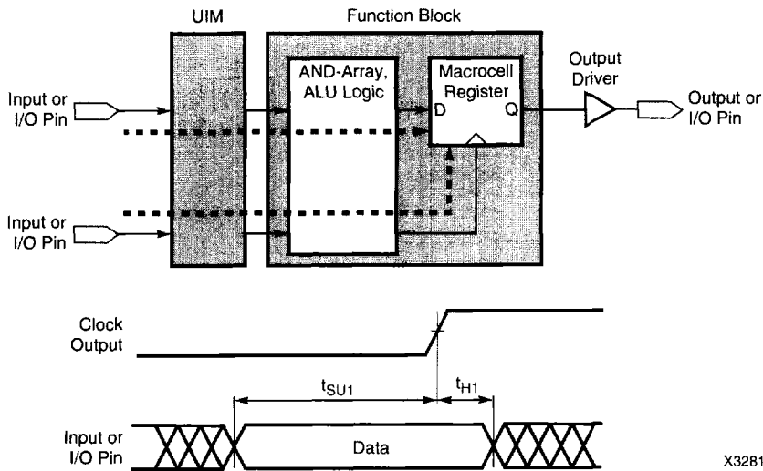
Figure 8: Delay Path Specification for t_{SU1} and t_{H1}
