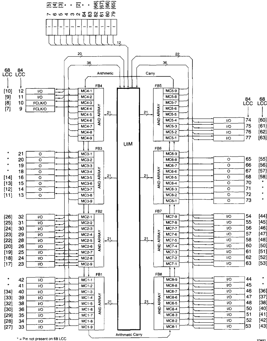
Figure 1: XC7272A Architecture
