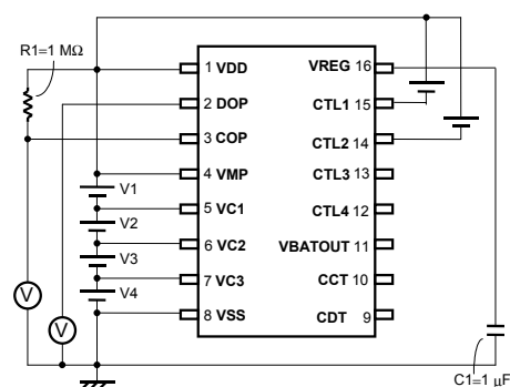
Test circuit 6
