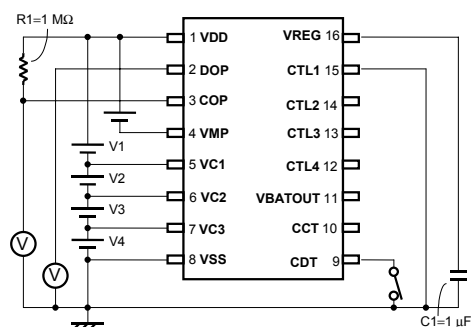
Test circuit 4
