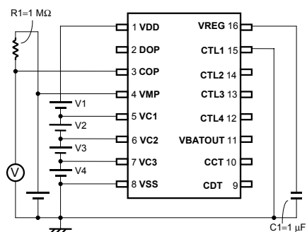
Test circuit 7
