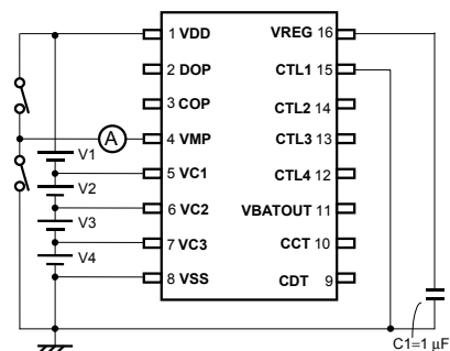
Test circuit 8
