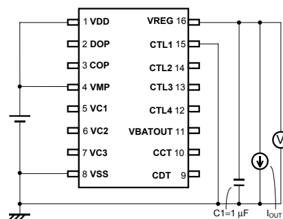
Test circuit 2
