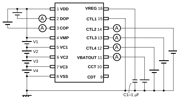
Test circuit 9
