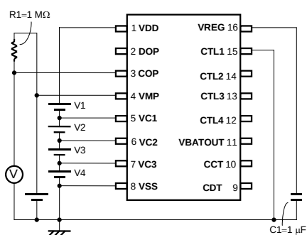
Test circuit 7
