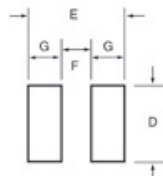
Recommended Solder Pad Layout
