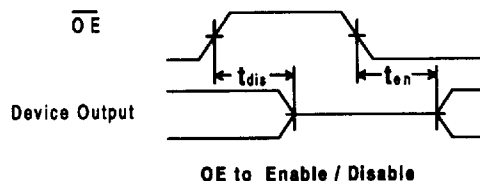
\overline{OE} to Enable / Disable
