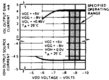
Output Current Versus VDD Supply Voltage
