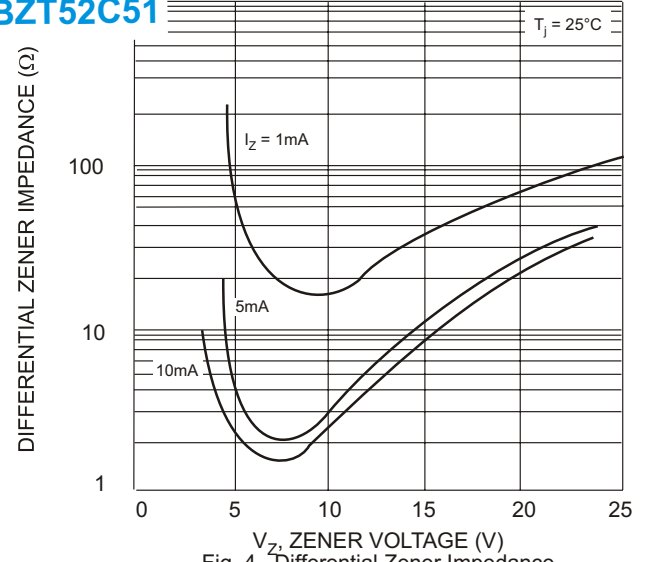
Fig. 4, Differential Zener Impedance
