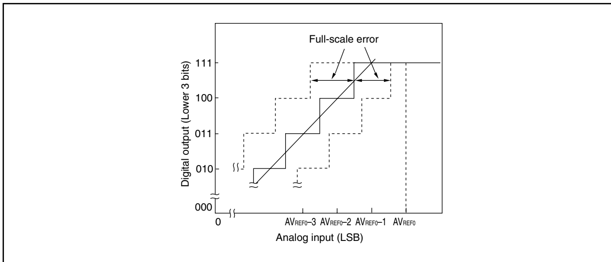
Figure 13-15. Full-Scale Error
