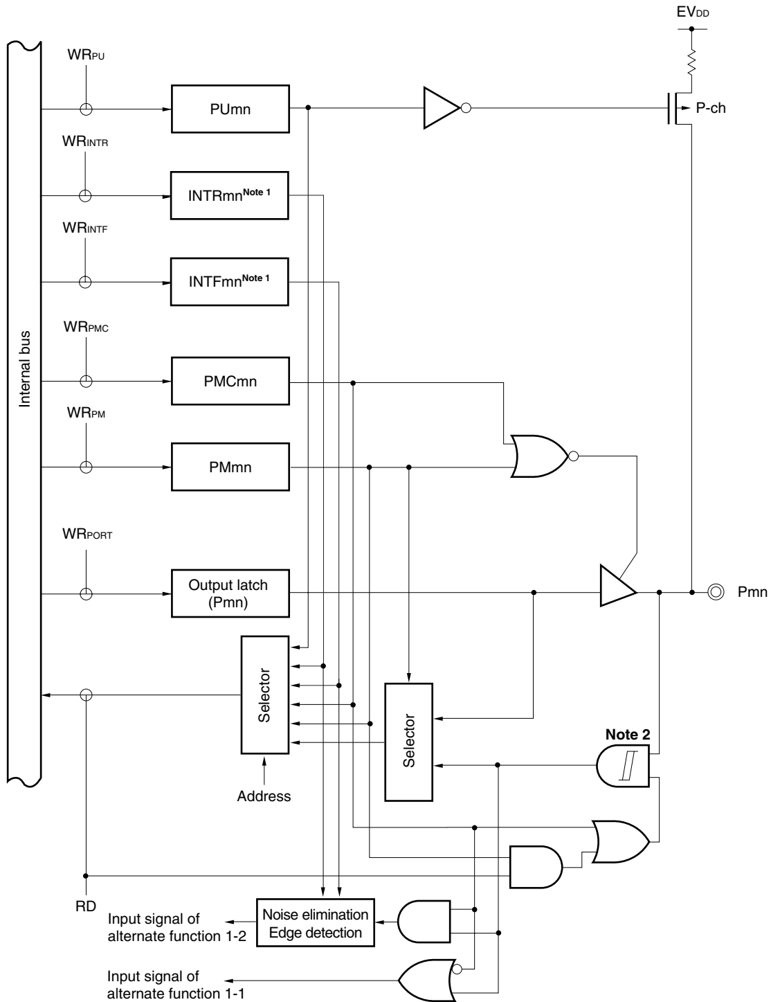
Figure 4-7. Block Diagram of Type D1-SUIHL
