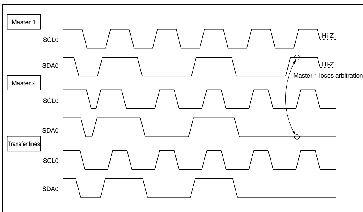
Figure 16-11. Arbitration Timing Example
