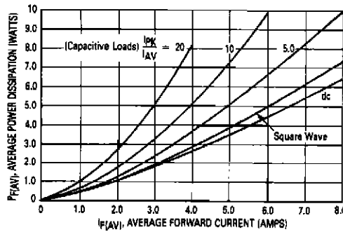
FIGURE 4 — POWER DISSIPATION
