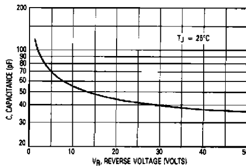
FIGURE 5 — TYPICAL CAPACITANCE
