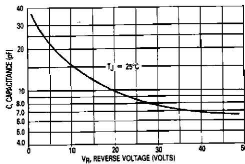
FIGURE 10 — TYPICAL CAPACITANCE
