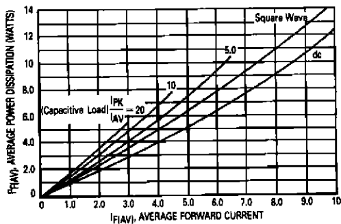
FIGURE 9 — POWER DISSIPATION
