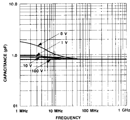
FIGURE 9. CAPACITANCE VS. FREQUENCY AND REVERSE BIAS - MA4P7100 SERIES
