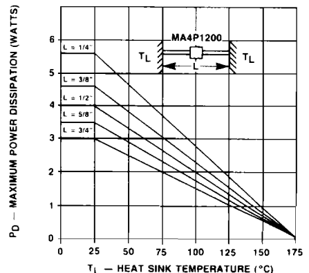
FIGURE 16. HEAT SINK TEMPERATURE VS. MAXIMUM POWER DISSIPATION – MA4P1200
