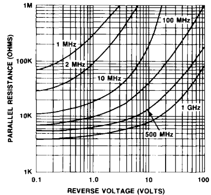
FIGURE 4. PARALLEL RESISTANCE VS. FREQUENCY AND REVERSE VOLTAGE – MA4P4000 SERIES
