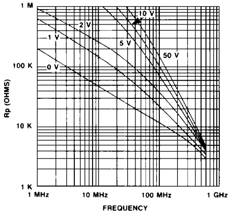
FIGURE 15. PARALLEL RESISTANCE VS. FREQUENCY AND REVERSE BIAS – MA4P1200 & MA4P1250
