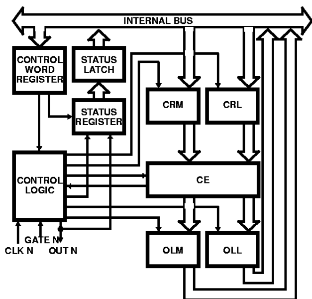
FIGURE 7. COUNTER INTERNAL BLOCK DIAGRAM
