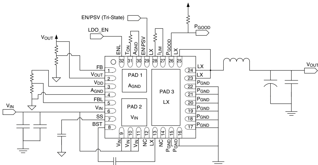
Typical Application Circuit for SiC401A/B (PowerPAK MLP5x5-32L)
