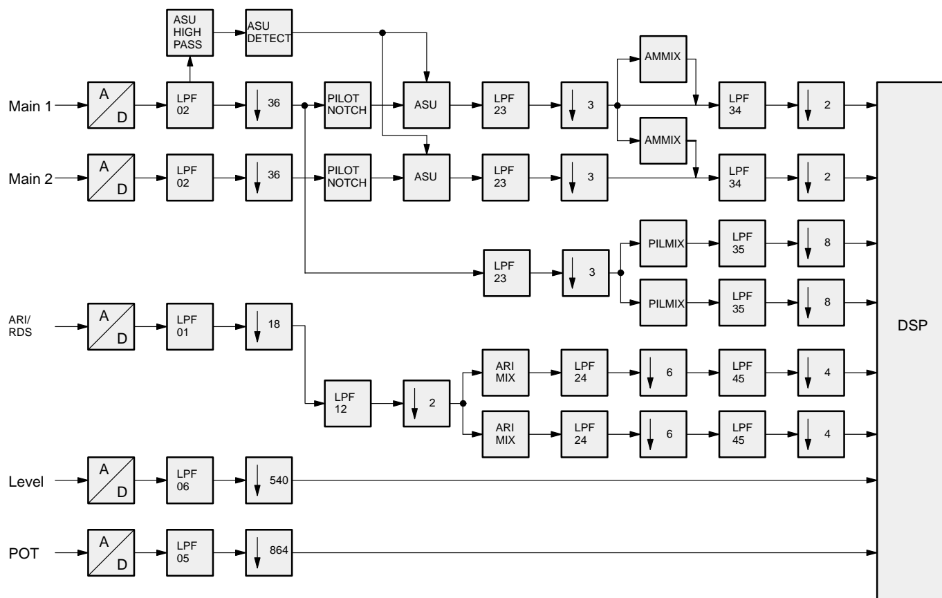
Fig. 2-5: Digital signal processing blocks, input side
