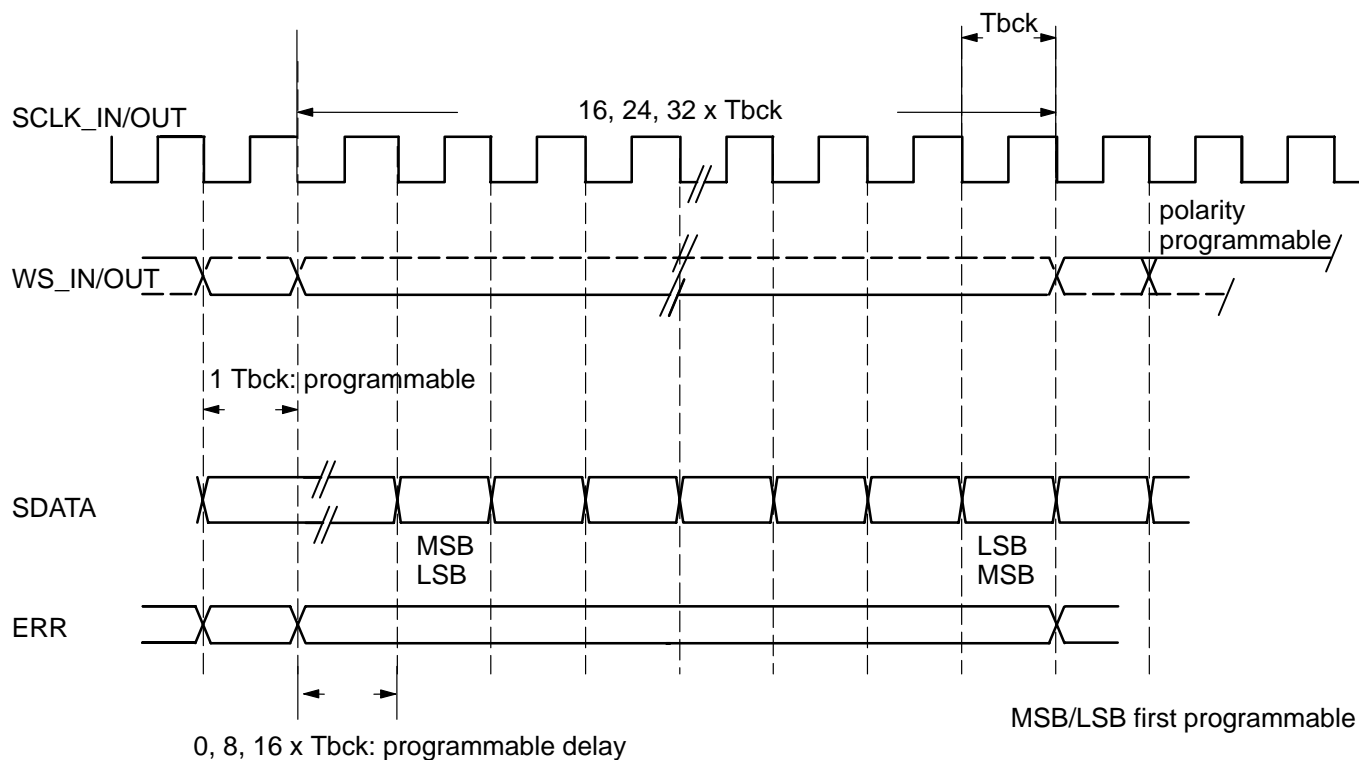
Fig. 2-13: Timing of the signals
