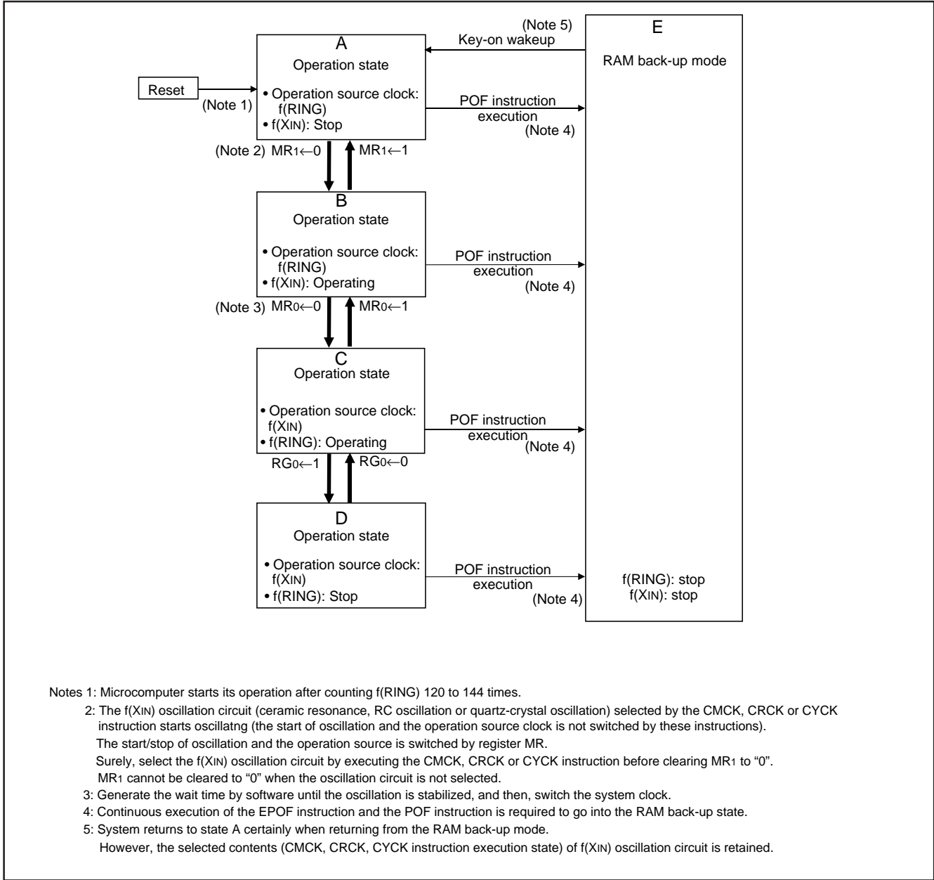
Fig. 51 State transition
