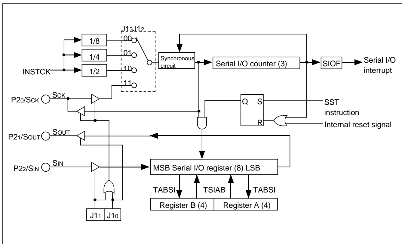
Fig. 40 Serial I/O structure
