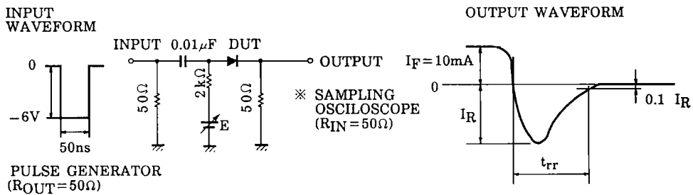
Fig. 1 REVERSE RECOVERY TIME ( t_{rr} ) TEST CIRCUIT
