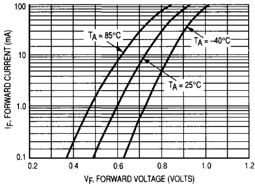
Figure 2. Forward Voltage
