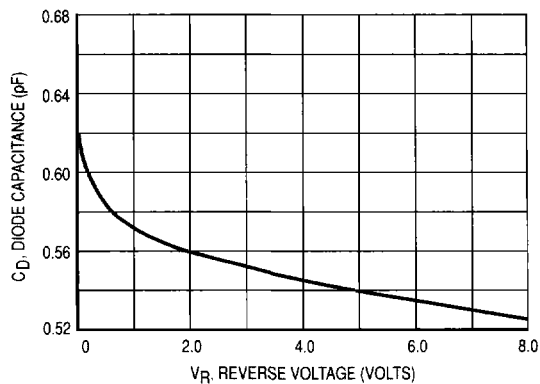
Figure 4. Capacitance
