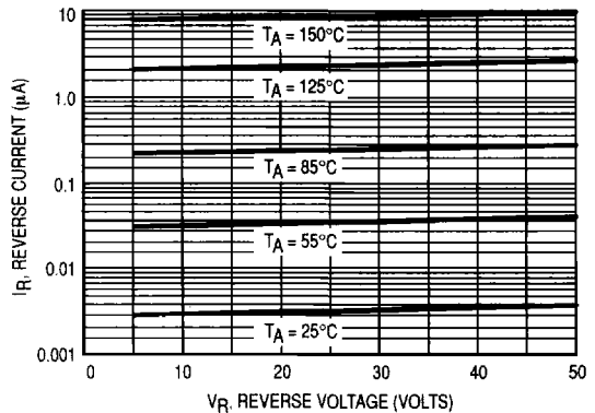
Figure 3. Leakage Current
