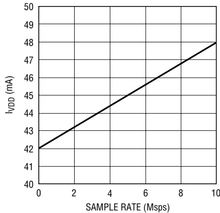
LTC2202: I_{VDD} vs Sample Rate, 5MHz Sine Wave, -1\text{dBFS}
