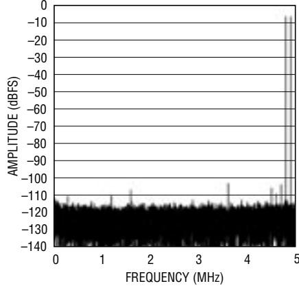
LTC2202: 32K Point FFT, f_{IN} = 5.1\text{MHz} and 15.2\text{MHz} , -7\text{dBFS} , \text{PGA} = 0
