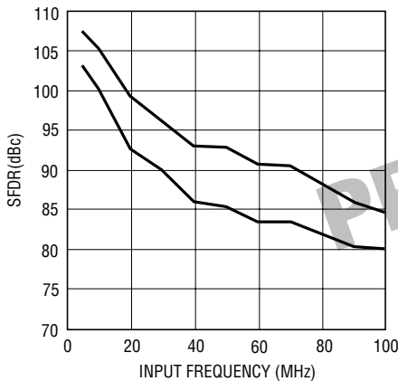
LTC2202: SFDR (HD2 and HD3) vs Input Frequency
