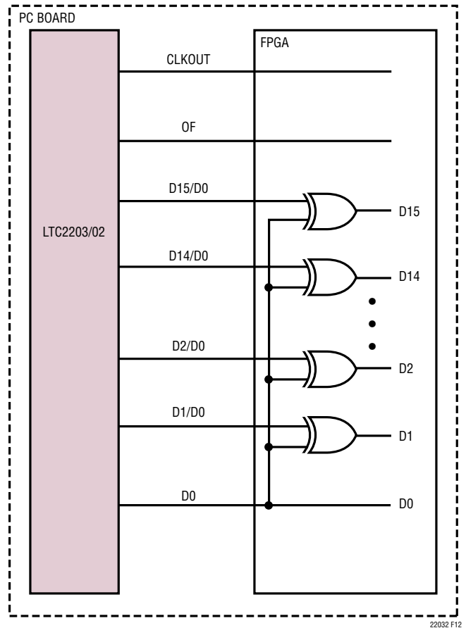
Figure 11. Descrambling a Scrambled Digital Output
