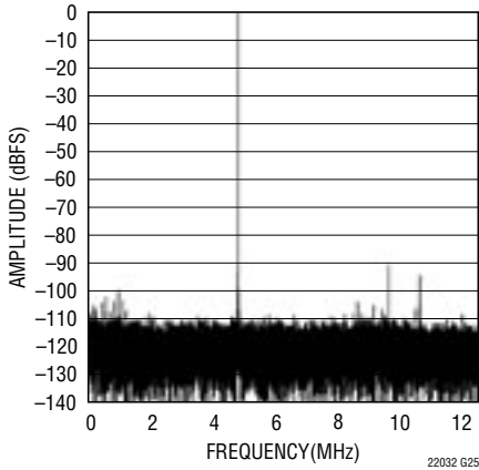
LTC2203: 32K Point FFT, f_{IN} = 70.1\text{MHz} , -1\text{dBFS} , PGA = 1
