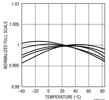
LTC2202: Normalized Full Scale vs Temperature, Internal Reference, 5 Units
