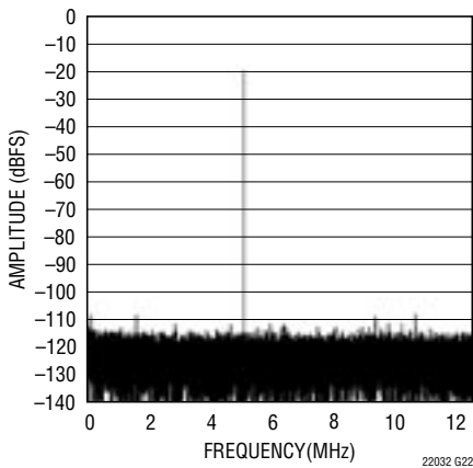
LTC2203: 32K Point FFT, f_{IN} = -30\text{MHz} , -20\text{dBFS} , PGA = 1
