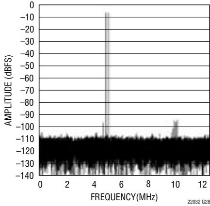
LTC2203: 32K Point FFT, f_{IN} = 44.9\text{MHz} and 70.1\text{MHz} , -7\text{dBFS} , \text{PGA} = 0
