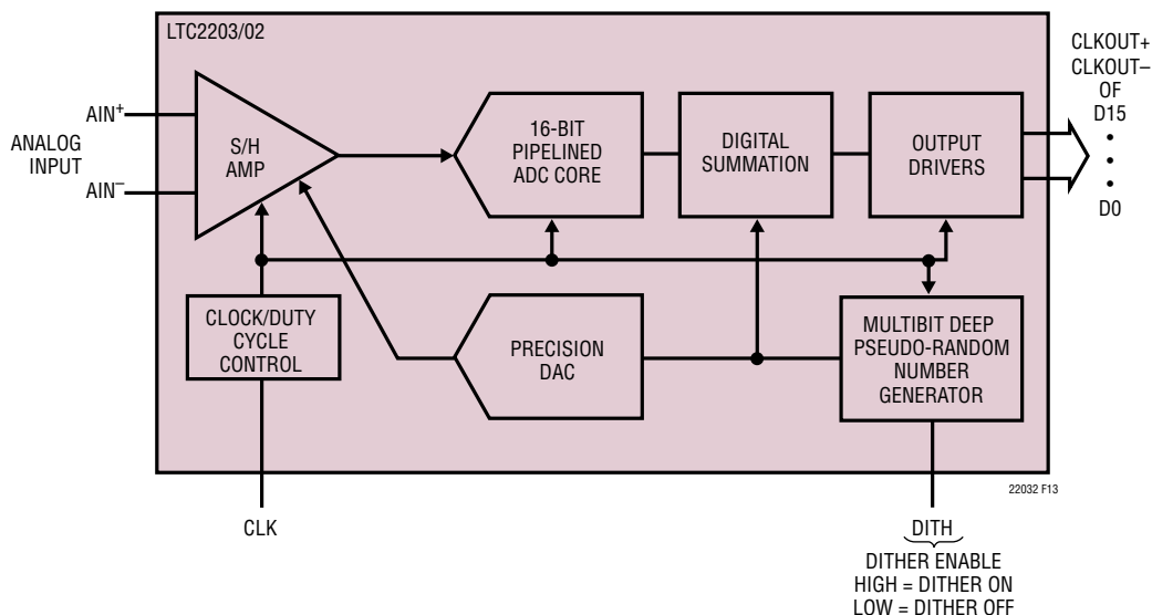
Figure 12. Functional Equivalent Block Diagram of Internal Dither Circuit
