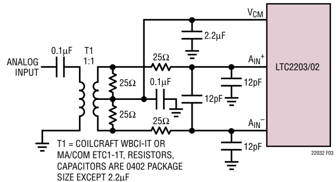
Figure 3. Single-Ended to Differential Conversion Using a Transformer. Recommended for Input Frequencies from 1MHz to 50MHz
