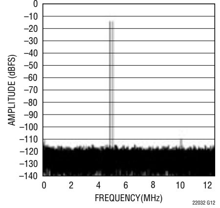
LTC2203: 32K Point FFT, f_{IN} = 4.9\text{MHz} and 30.1\text{MHz} , -15\text{dBFS} , \text{PGA} = 0
