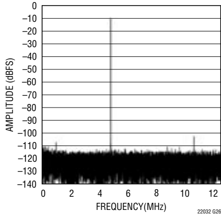
LTC2203: 32K Point FFT, f_{IN} = 70.1\text{MHz} , -10\text{dBFS} , PGA = 1
