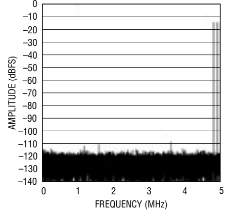
LTC2202: 32K Point FFT, f_{IN} = 5.1\text{MHz} and 15.2\text{MHz} , -15\text{dBFS} , \text{PGA} = 0
