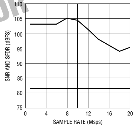
LTC2202: SNR and SFDR vs Sample Rate
