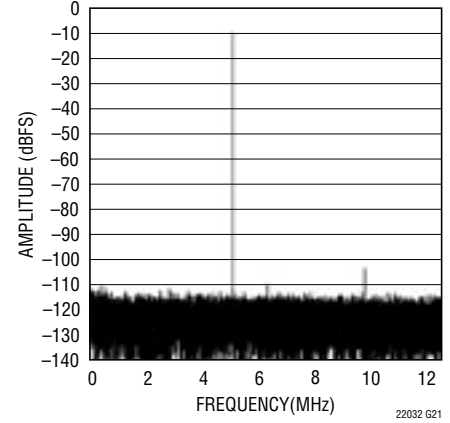
LTC2203: 32K Point FFT, f_{IN} = 30\text{MHz} , -10\text{dBFS} , PGA = 1
