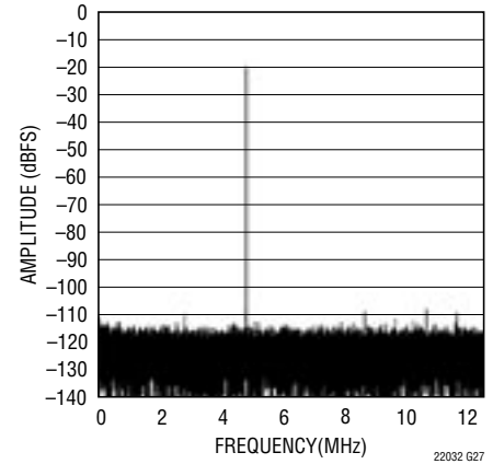
LTC2203: 32K Point FFT, f_{IN} = 70.1\text{MHz} , -20\text{dBFS} , PGA = 1
