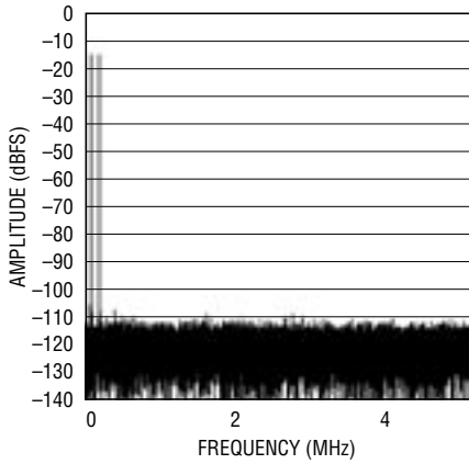
LTC2202: 32K Point FFT, f_{IN} = 60.2\text{MHz} and 70.1\text{MHz} , -15\text{dBFS} , \text{PGA} = 0
