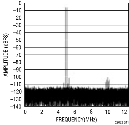
LTC2203: 32K Point FFT, f_{IN} = 4.9\text{MHz} and 30.1\text{MHz} , -7\text{dBFS} , \text{PGA} = 0
