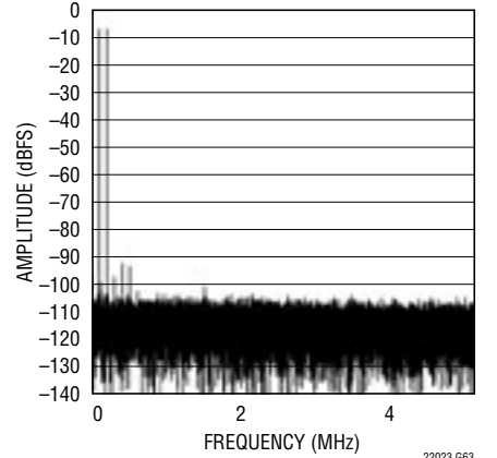
LTC2202: 32K Point FFT, f_{IN} = 60.2\text{MHz} and 70.1\text{MHz} , -7\text{dBFS} , \text{PGA} = 0
