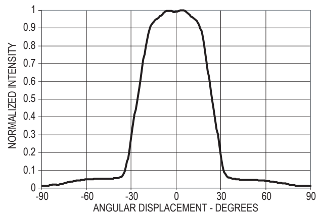
Figure 10. Radiation Pattern
