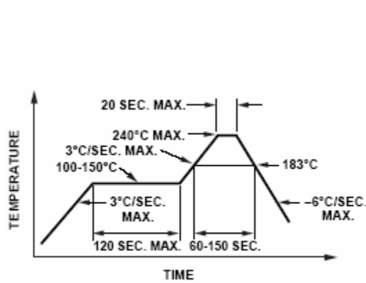
Figure 11a. Recommended SnPb Reflow Soldering Profile.
