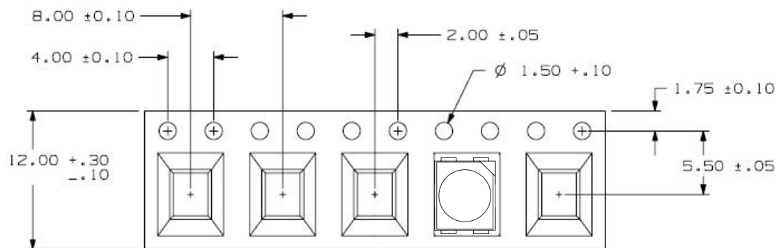
Figure 15. Tape Dimensions
