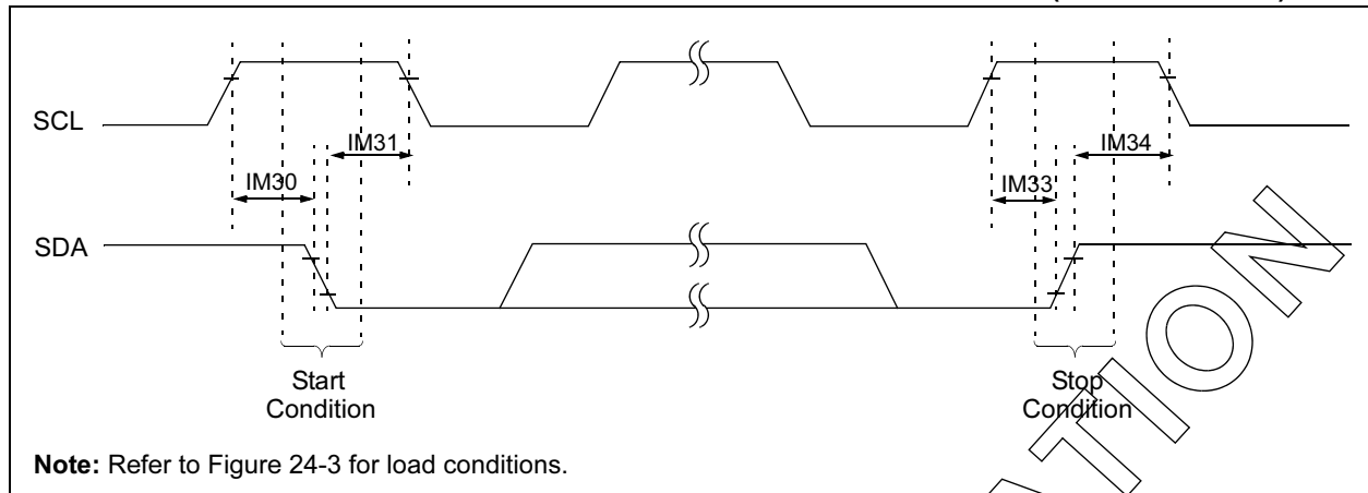
FIGURE 24-24: I 2 C BUS DATA TIMING CHARACTERISTICS (MASTER MODE)
