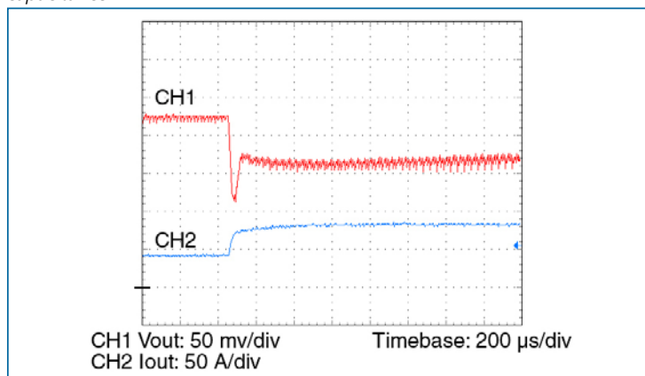
Figure 4-5 – Transient response 50 – 100%, 3 x 4.7 µF ceramic bypass capacitance
