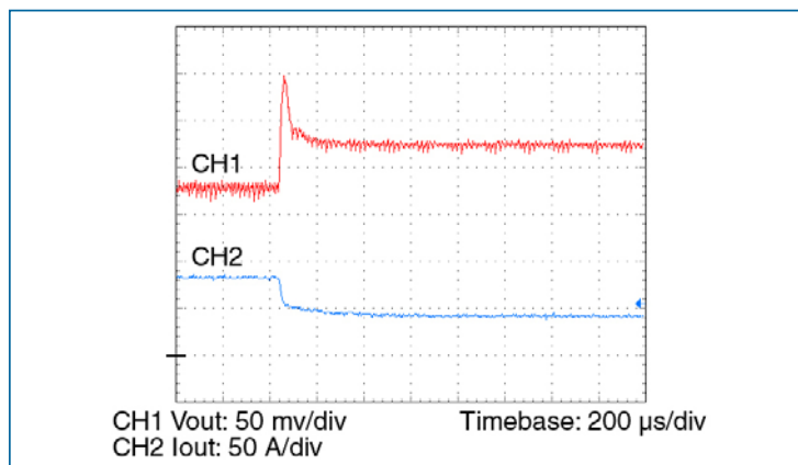
Figure 4-4 – Transient response 100 – 50%, 3 x 4.7 µF ceramic bypass capacitance
