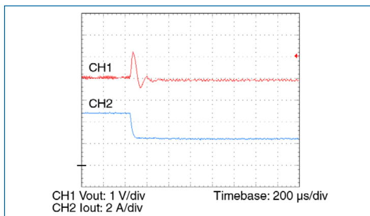
Figure 14-4 – Transient response 100 – 50%, 3 x 4.7 µF ceramic bypass capacitance
