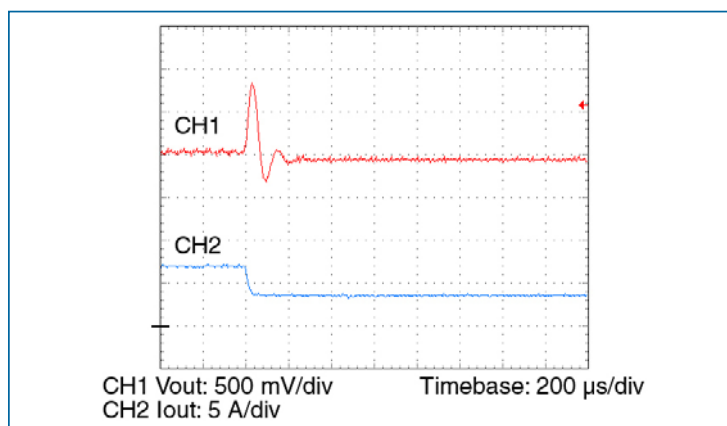
Figure 13-4 – Transient response 100 – 50%, 3 x 4.7 µF ceramic bypass capacitance
