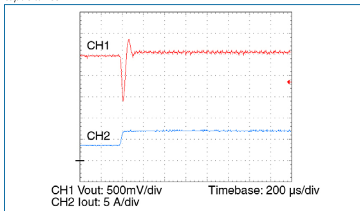
Figure 13-5 – Transient response 50 – 100%, 3 x 4.7 µF ceramic bypass capacitance
