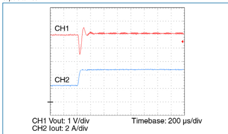
Figure 14-5 – Transient response 50 – 100%, 3 x 4.7 µF ceramic bypass capacitance
