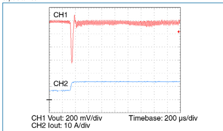
Figure 11-5 – Transient response 50 – 100%, 3 x 4.7 µF ceramic bypass capacitance
