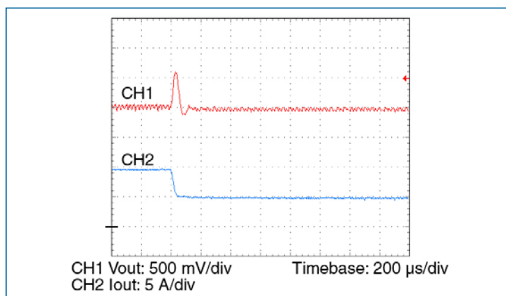
Figure 12-4 – Transient response 100 – 50%, 3 x 4.7 µF ceramic bypass capacitance
