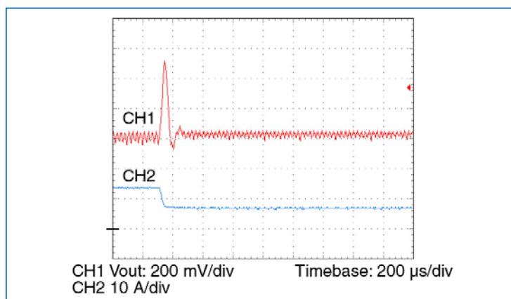
Figure 11-4 – Transient response 100 – 50%, 3 x 4.7 µF ceramic bypass capacitance
