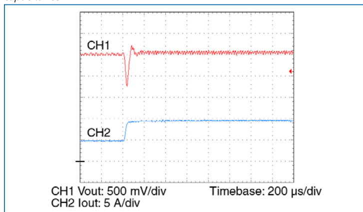
Figure 12-5 – Transient response 50 – 100%, 3 x 4.7 µF ceramic bypass capacitance
