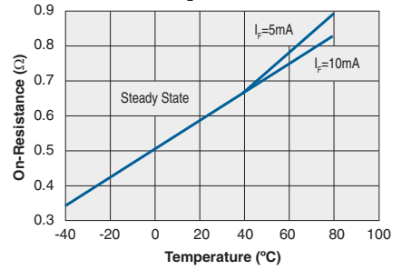
Typical On-Resistance vs. Temperature ( I_L=480\text{mA} )
