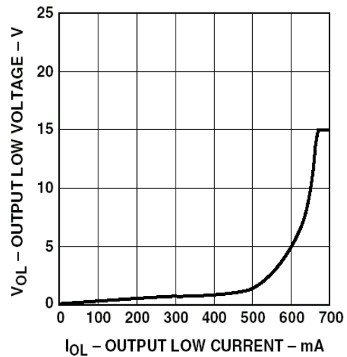
Figure 6. V_{OL} vs. I_{OL} .
