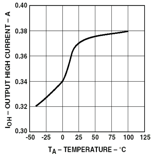
Figure 2. I_{OH} vs. Temperature.
