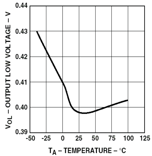
Figure 4. V_{OL} vs. Temperature.
