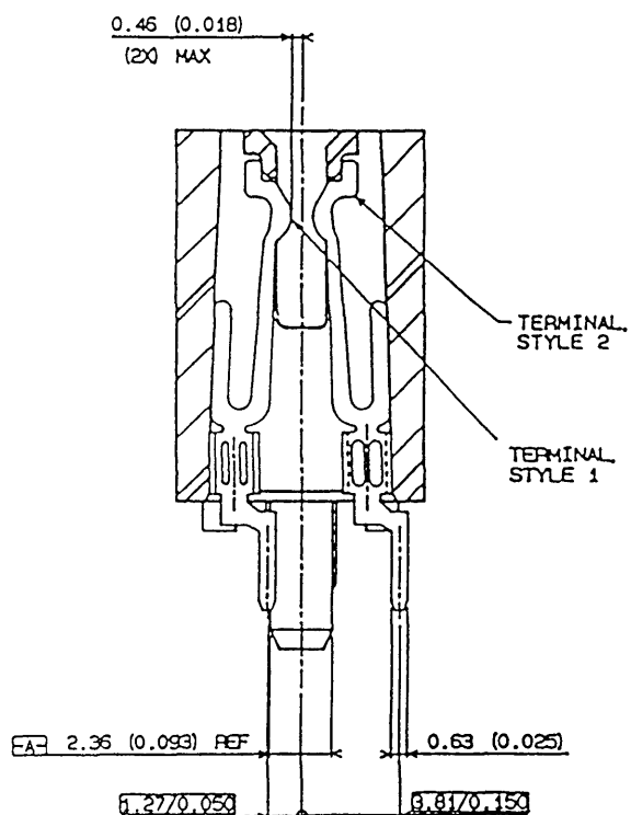
SECTION Y-Y ROTATED 90° CW
