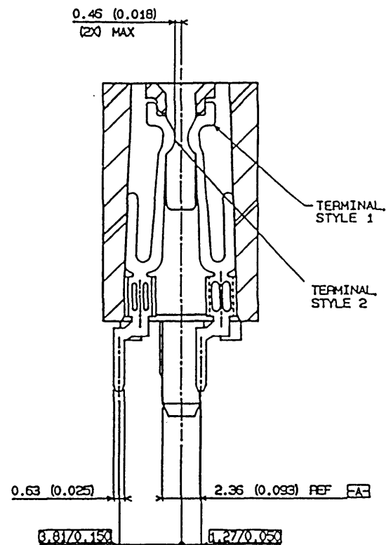
SECTION X-X ROTATED 90° CW
