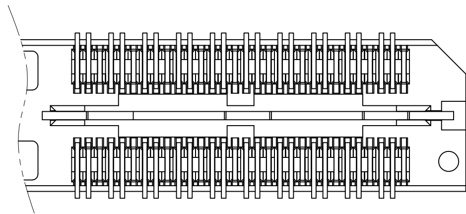
DIFFERENTIAL PAIR CONTACT ARRANGEMENT (BOTTOM VIEW) SCALE 2:1
