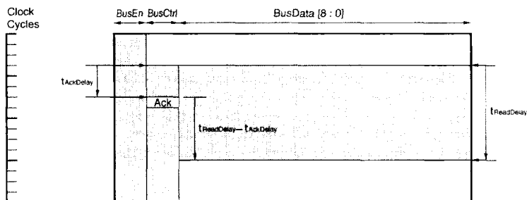
Figure 7-1. Read Transaction
