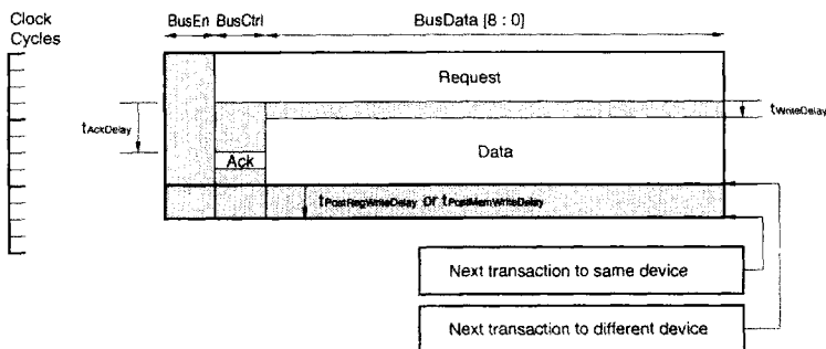
Figure 7-2. Write Transaction
