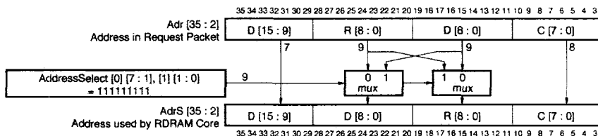
Figure 9-1. AddressMapping Hardware
