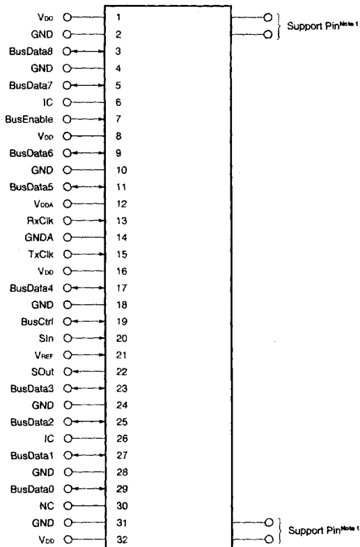
Figure Support Pin Diagram
