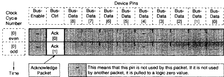
Figure 5-2. Acknowledge Packet Format
