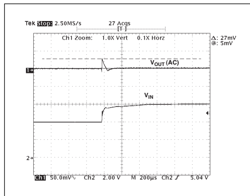
Line Regulation, Line Step from 4V to 6V, I_O = 1\text{mA}
