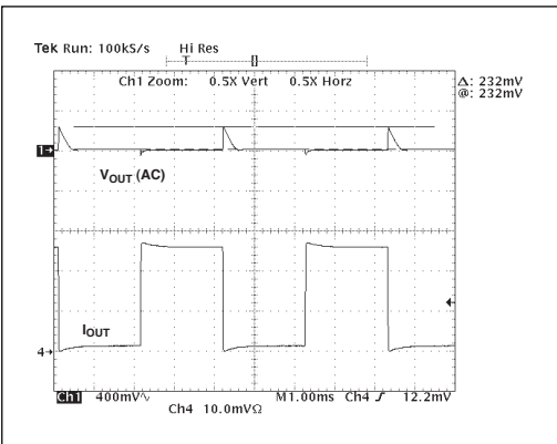
Load Regulation, I_O = 100\mu\text{A} \sim 500\text{mA}
