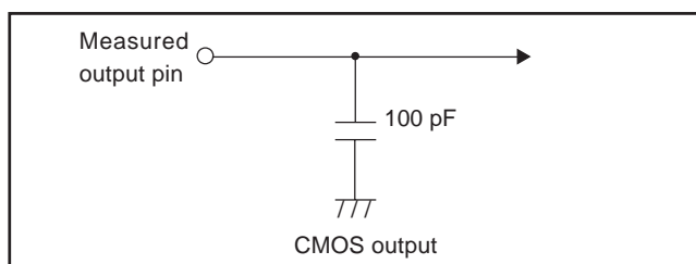
Switching characteristics measurement circuit diagram (Extended operating temperature version)
