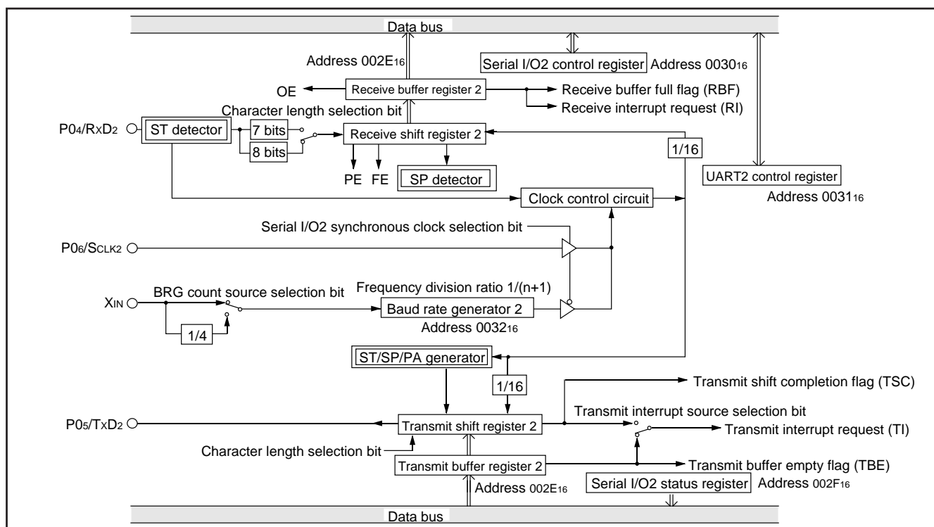
Fig. 62 Block diagram of UART serial I/O2
