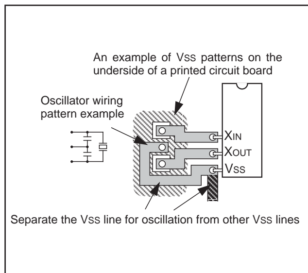
Fig. 91 Vss pattern on the underside of an oscillator
