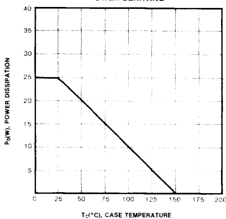
POWER DERATING
