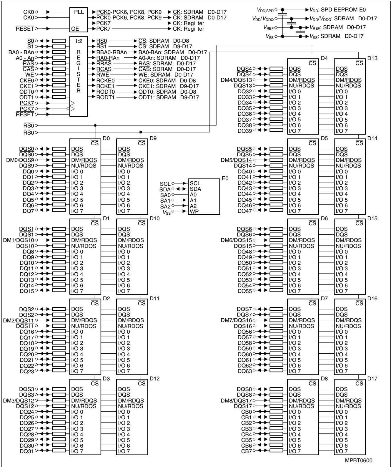
Figure 3 Block Diagram Raw Card G RDIMM (x72, 2 Ranks, x8)
