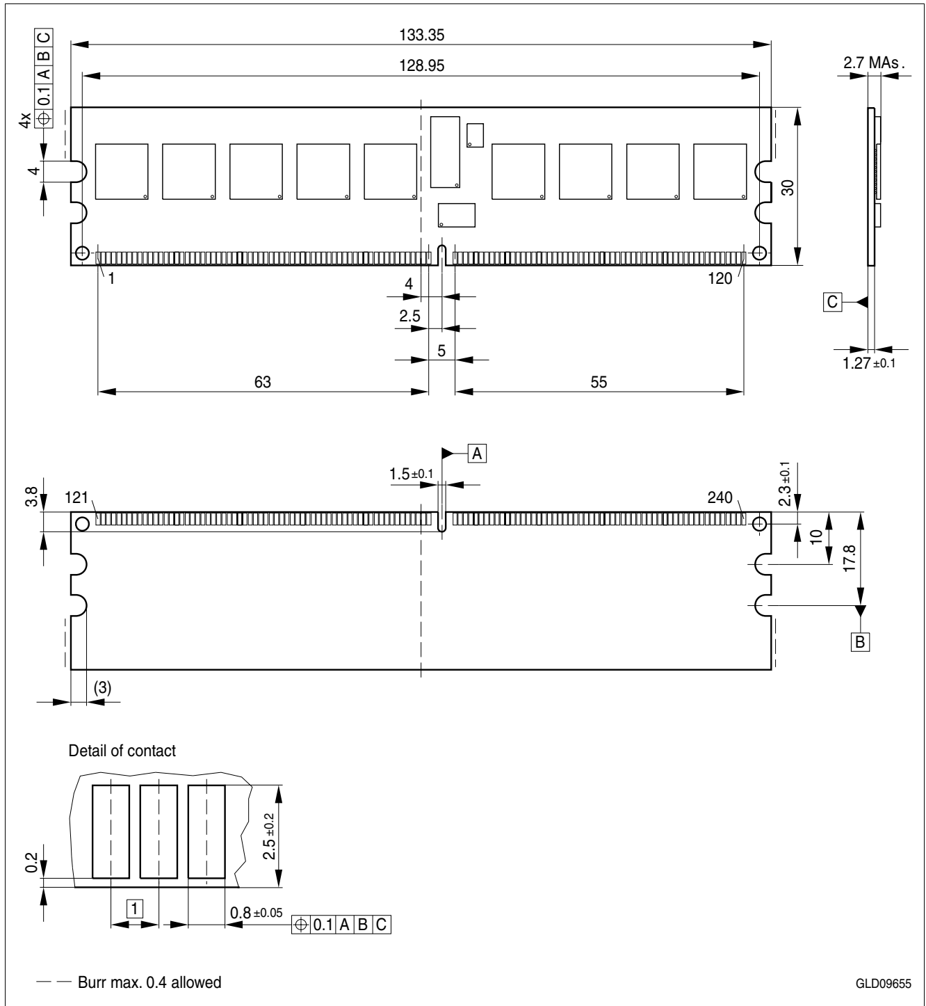
Figure 8 Package Outline Raw Card F L-DIM-240-11
