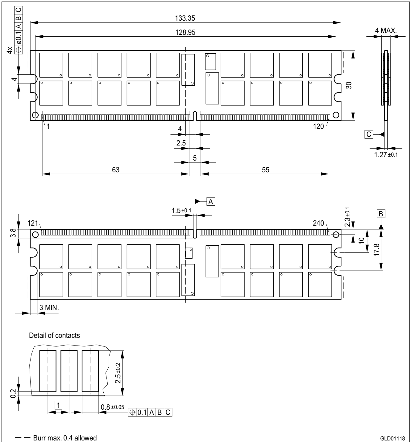
Figure 13 Package Outline Raw Card N L-DIM-240-44
