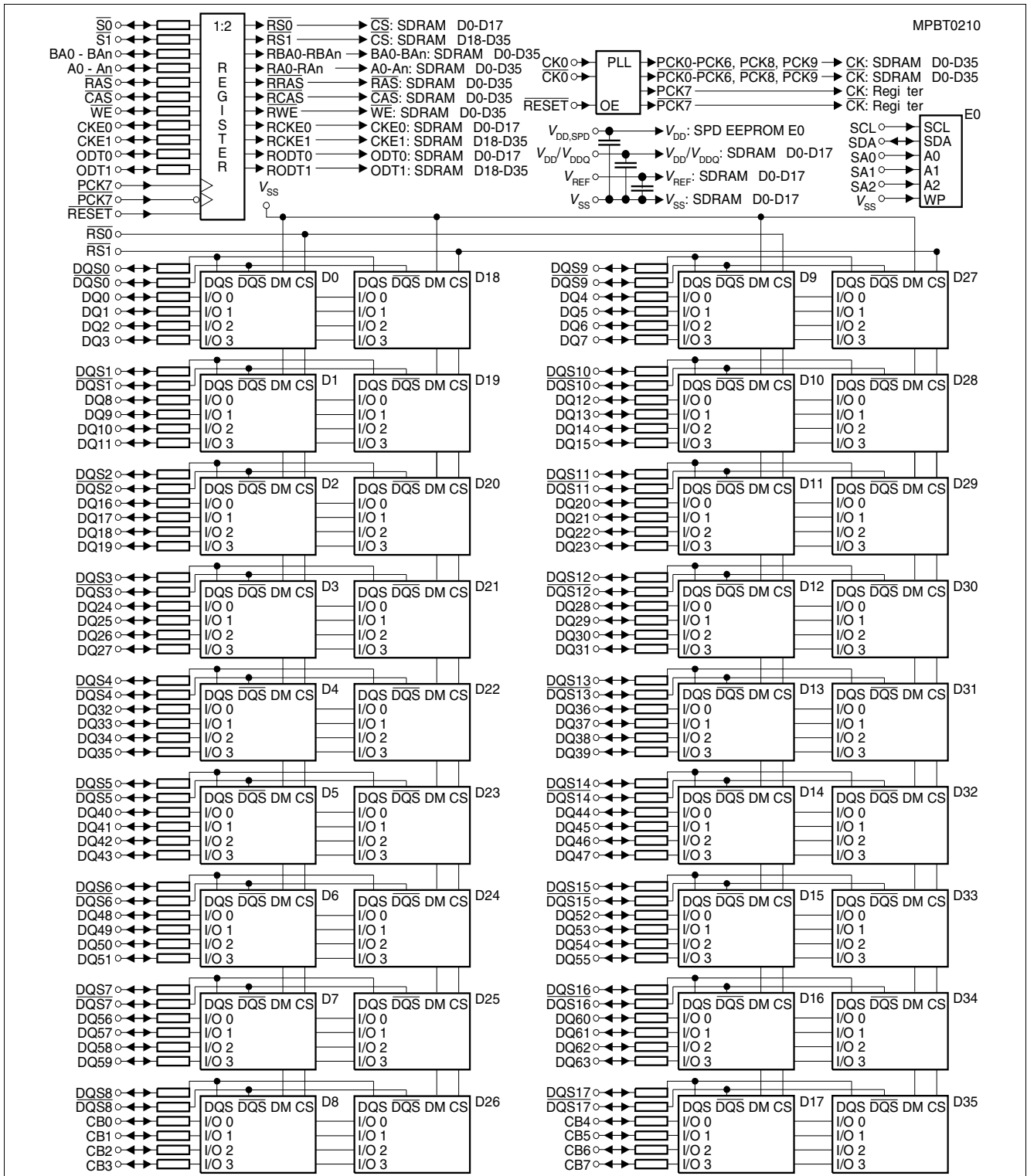
Figure 5 Block Diagram Raw Card L RDIMM (x72, 2Ranks, x4)
