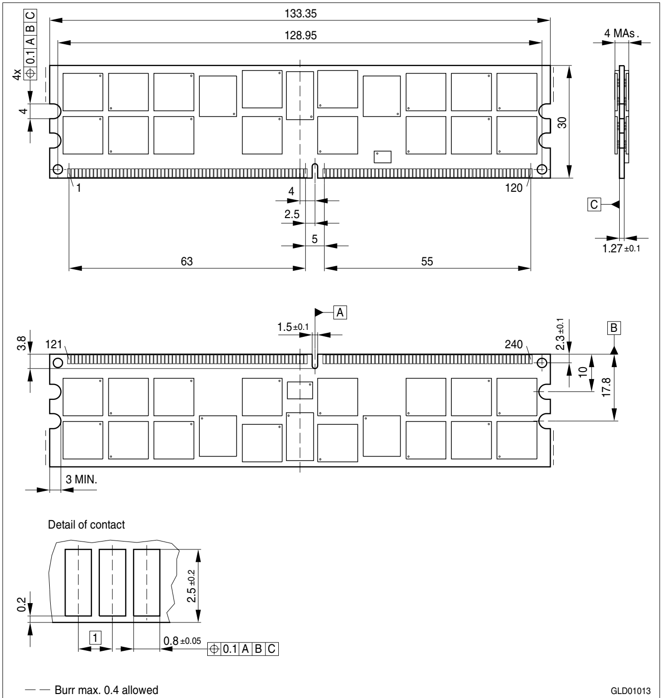
Figure 12 Package Outline Raw Card L L-DIM-240-40
