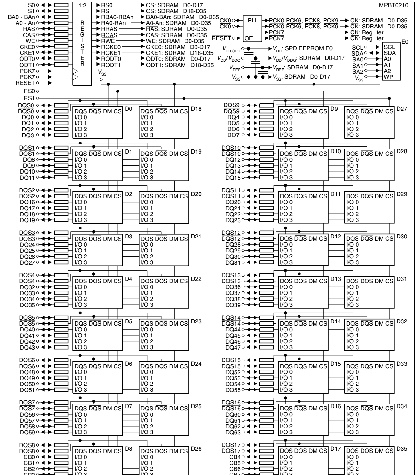
Figure 6 Block Diagram Raw Card J RDIMM (x72, 2Ranks, x4)
