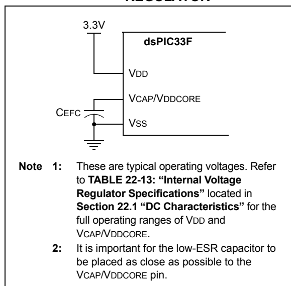
FIGURE 19-1: CONNECTIONS FOR THE ON-CHIP VOLTAGE REGULATOR (1)
